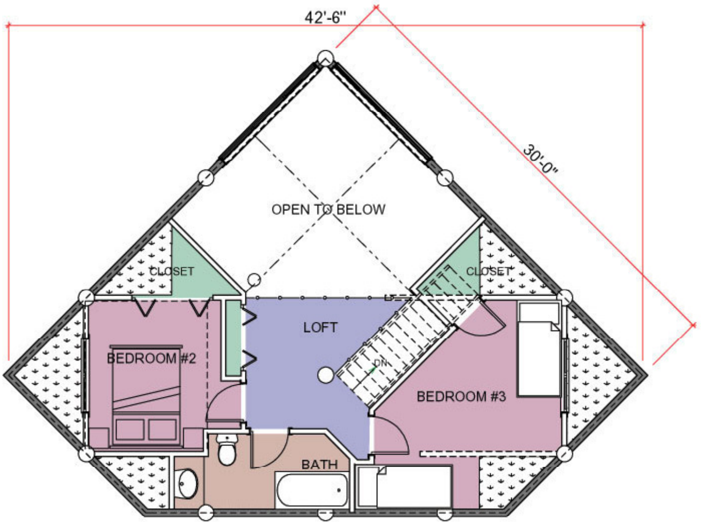
SECOND FLOOR PLAN AREA: 367 SQ. FT.
